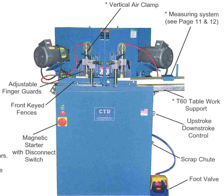
Model D45AX Automatic * Optional Extras Available
