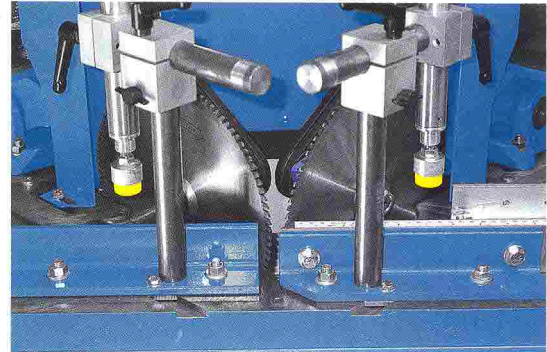
Fence & Blade Configuration
